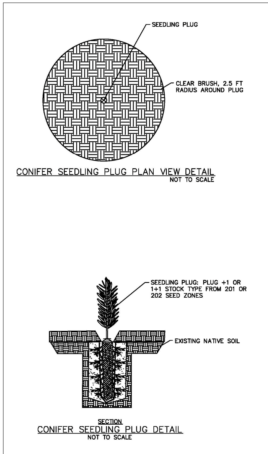
Figure B. 10. Wetland Enhancement Design Details – Conifer Seedling/Underplanting
